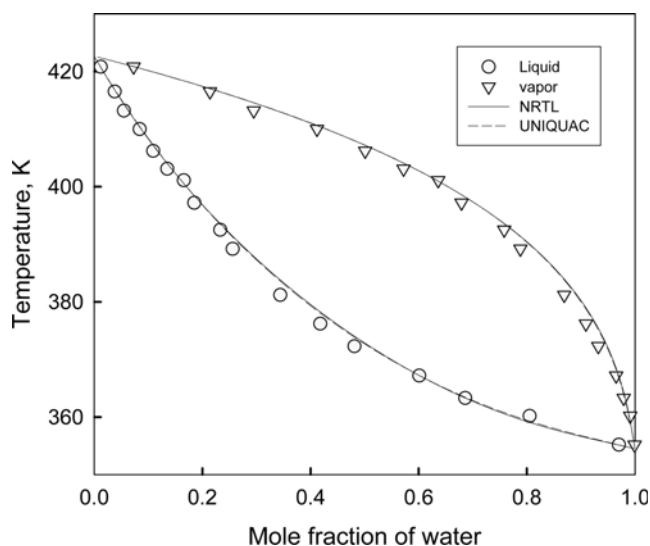
Fig. 5. Vapor liquid equilibrium of water+monoethanolamine system at 50.0 kPa.
